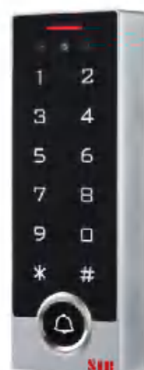
3D-TB2 134*48*23mm
