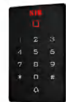
K12 114*75*16mm
