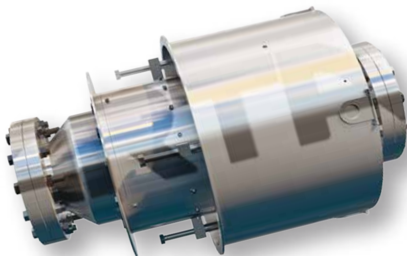
NTS®-MP PERC Safety Breakaway Couplings
